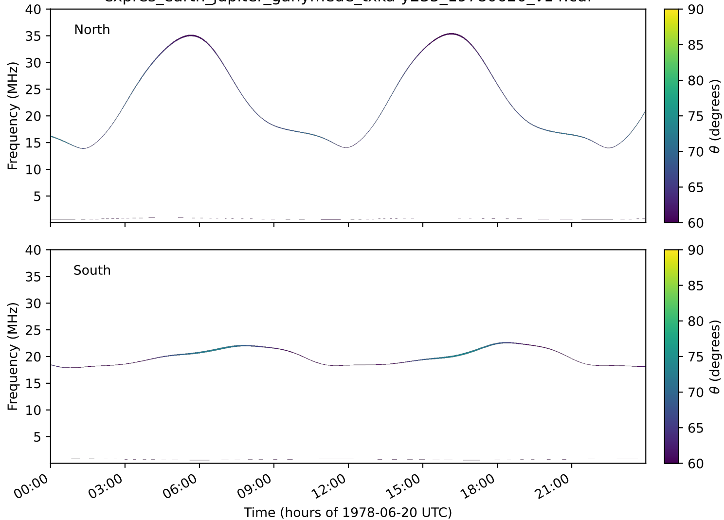
expres_earth_jupiter_ganymede_txka-y235_19780620_v14.cdf
