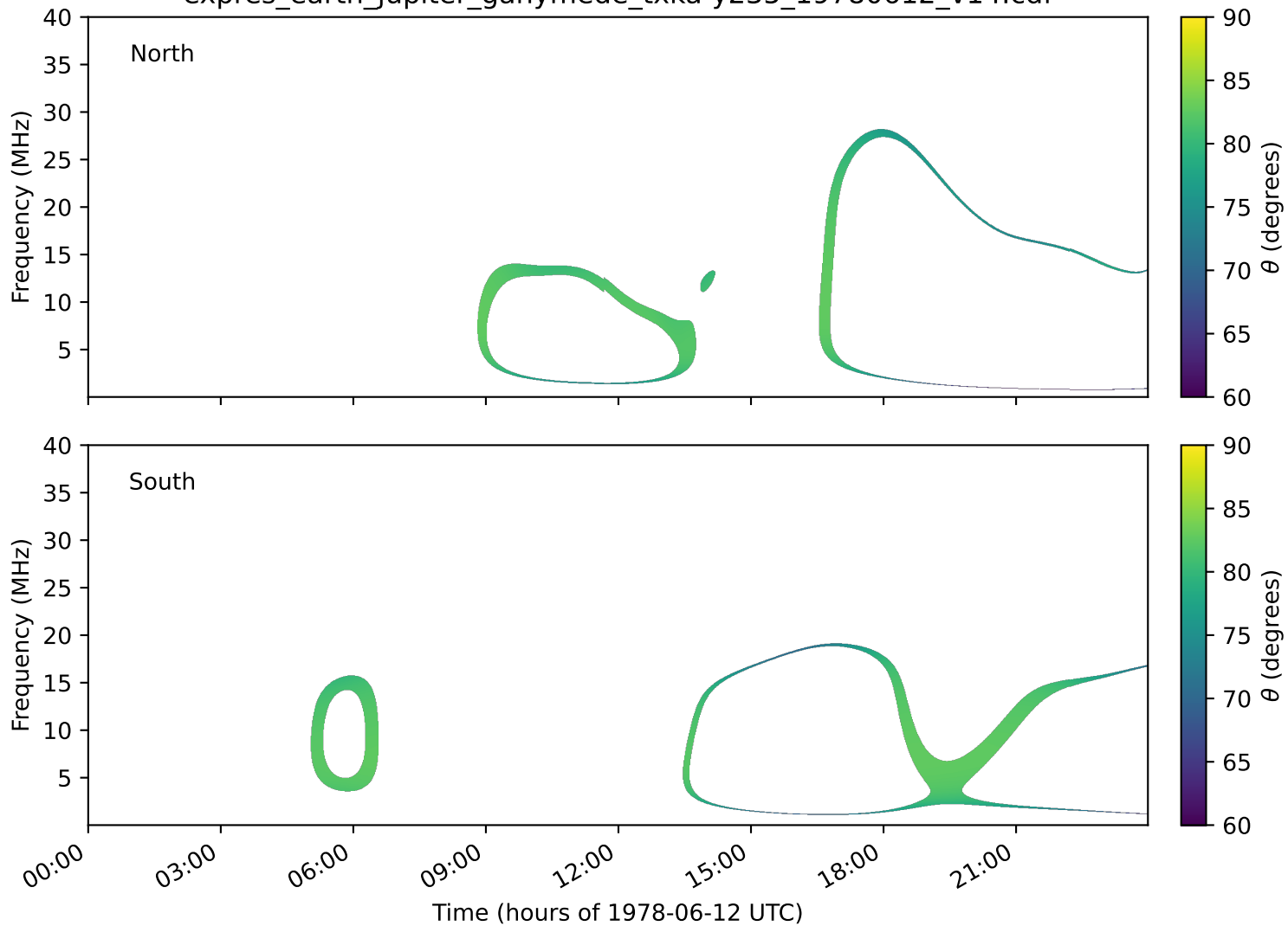
expres_earth_jupiter_ganymede_txka-y235_19780612_v14.cdf
