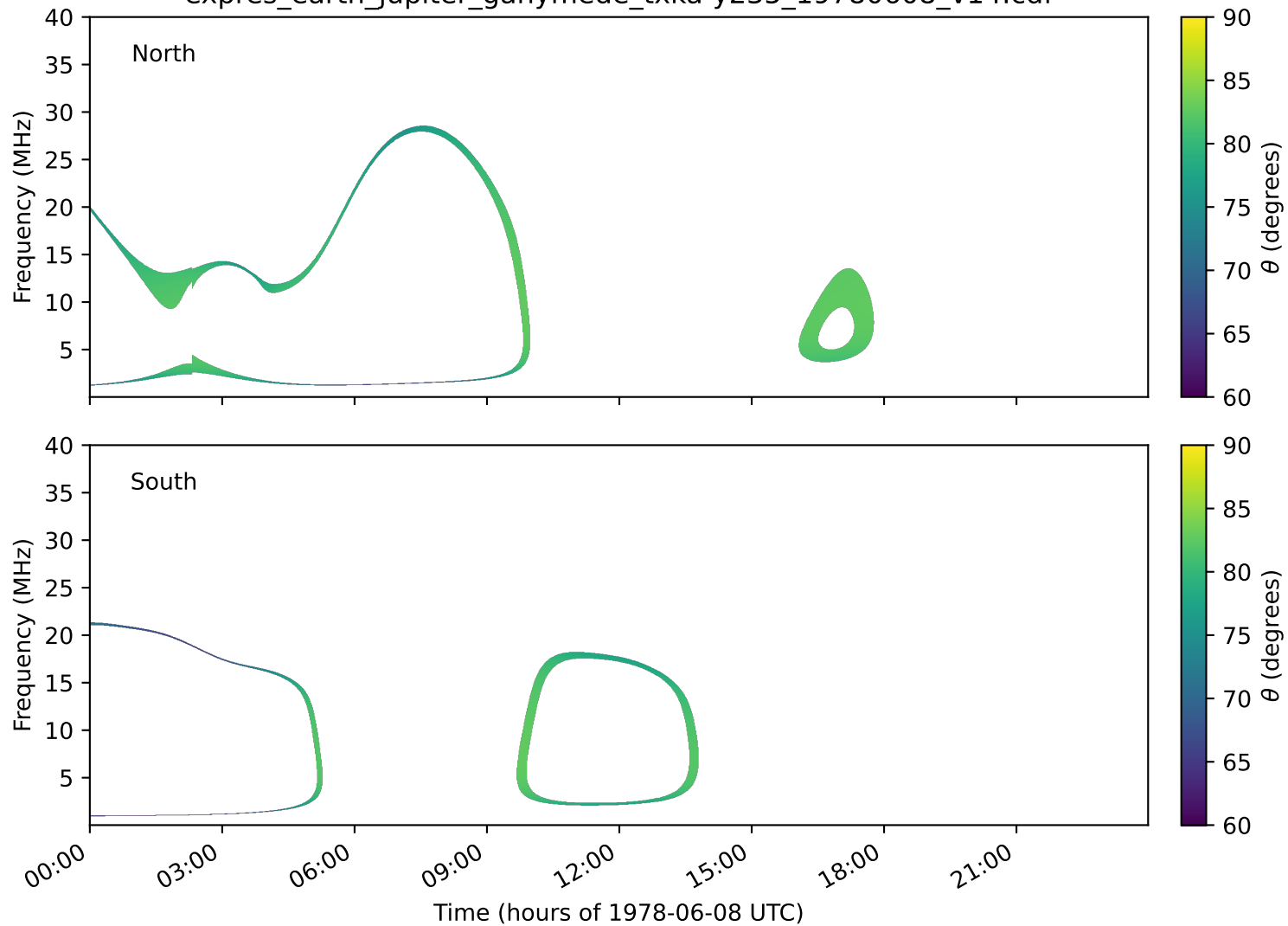
expres_earth_jupiter_ganymede_txka-y235_19780608_v14.cdf
