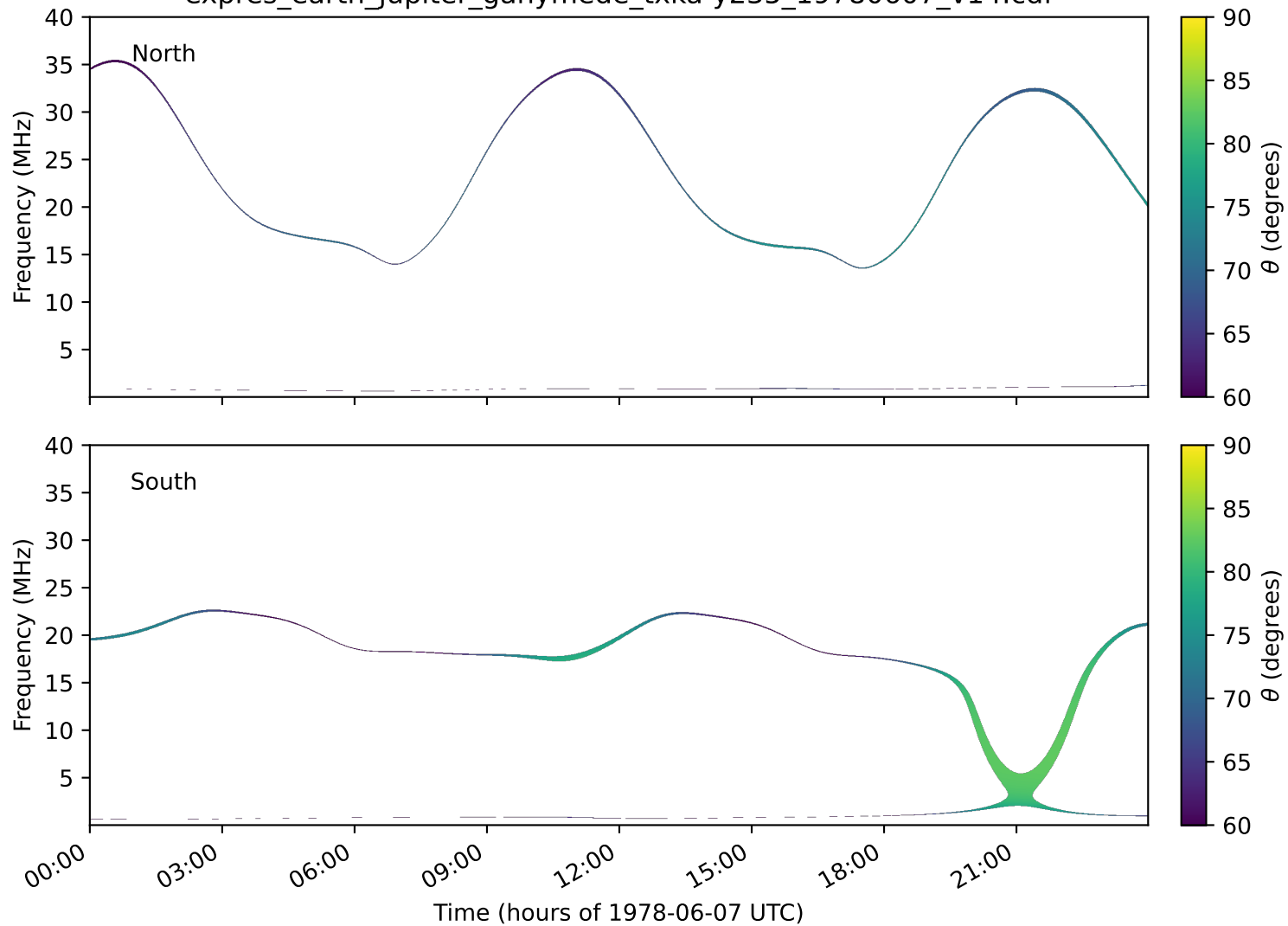
expres_earth_jupiter_ganymede_txka-y235_19780607_v14.cdf
