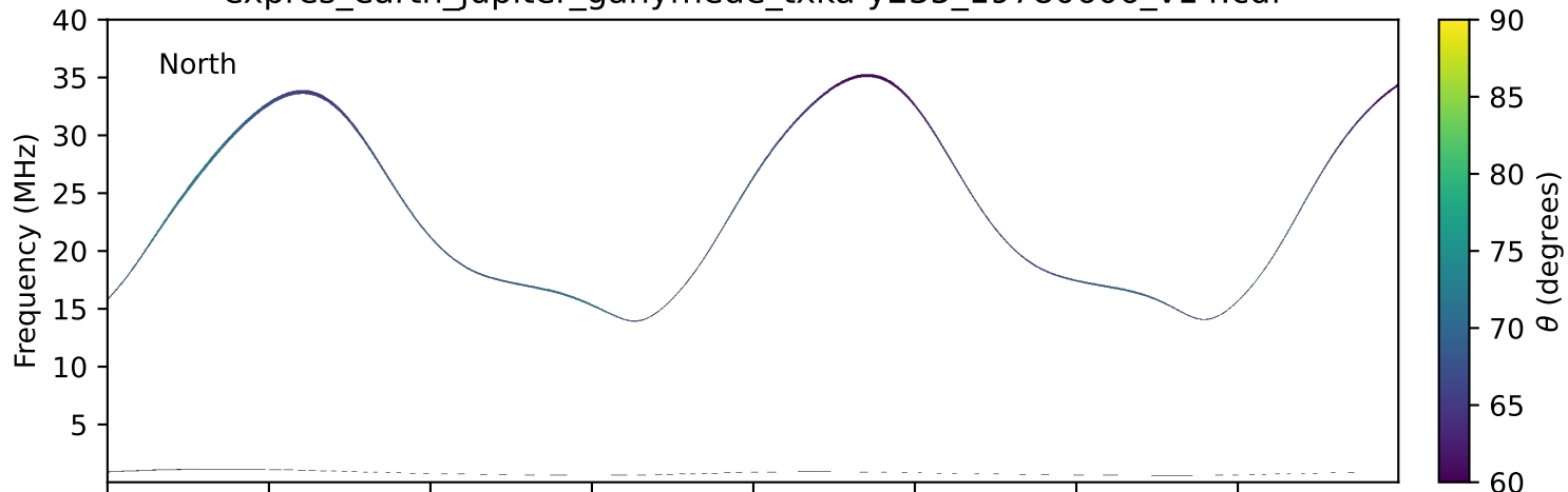
expres_earth_jupiter_ganymede_txka-y235_19780606_v14.cdf
