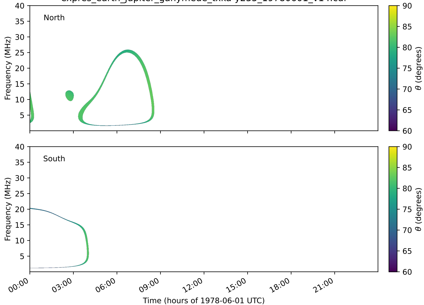
expres_earth_jupiter_ganymede_txka-y235_19780601_v14.cdf
