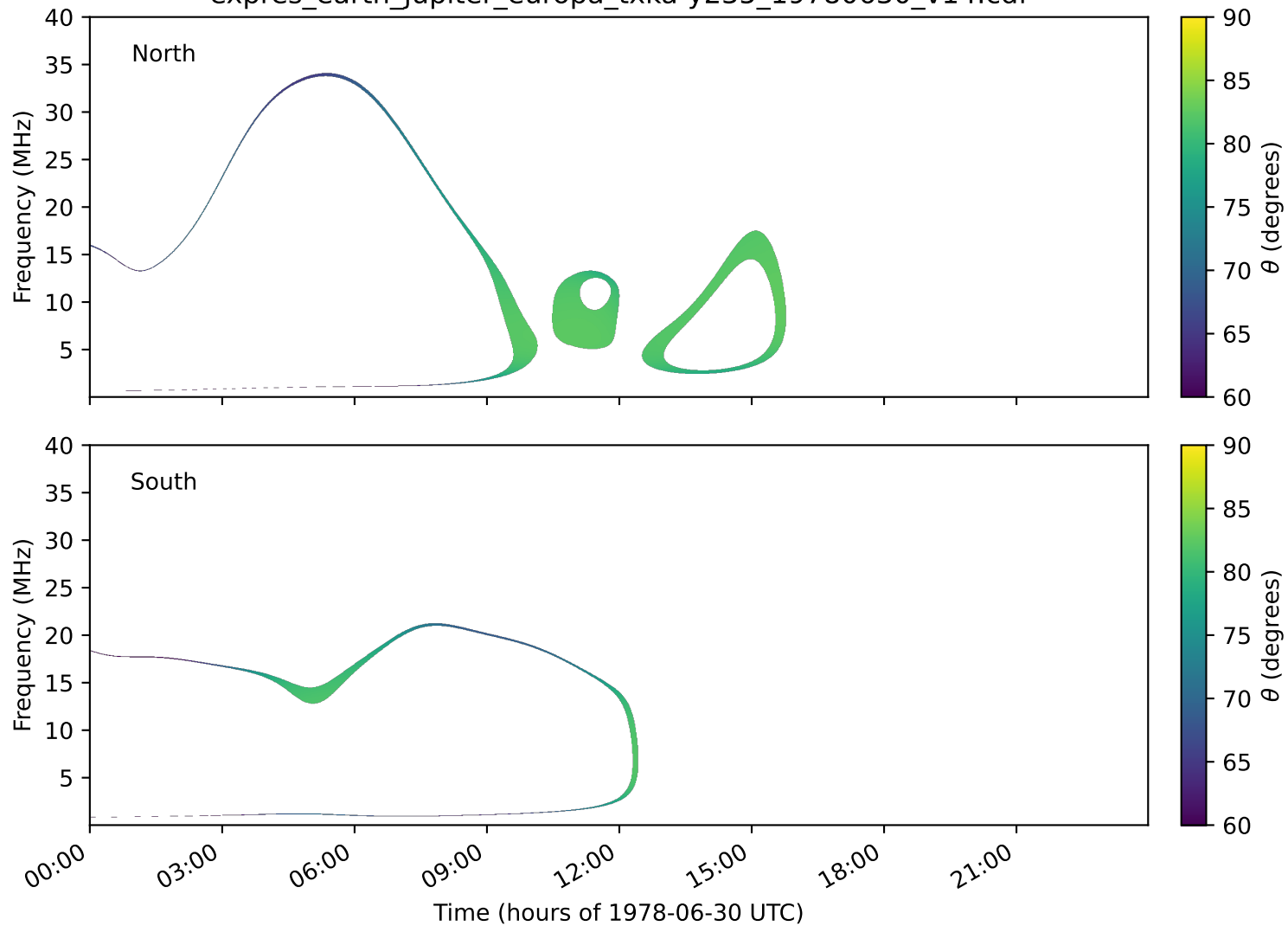
expres_earth_jupiter_europa_txka-y235_19780630_v14.cdf
