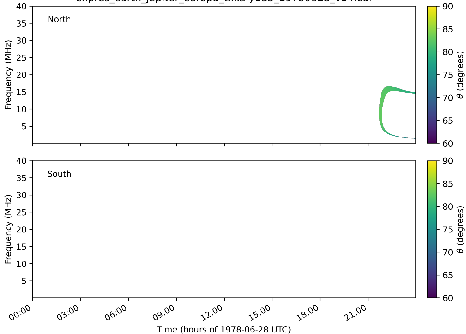
expres_earth_jupiter_europa_txka-y235_19780628_v14.cdf
