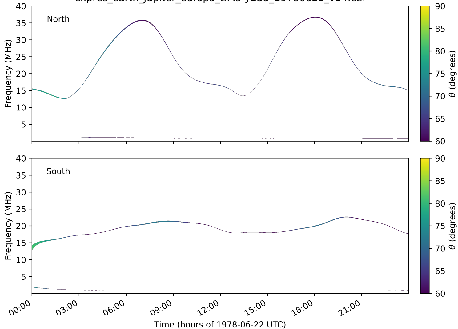
expres_earth_jupiter_europa_txka-y235_19780622_v14.cdf
