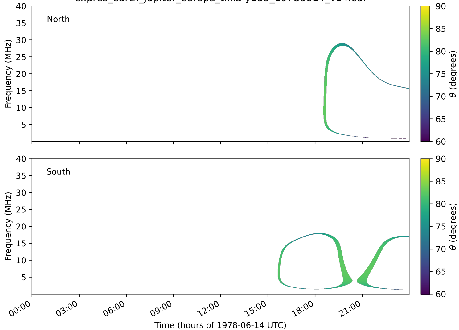
expres_earth_jupiter_europa_txka-y235_19780614_v14.cdf
