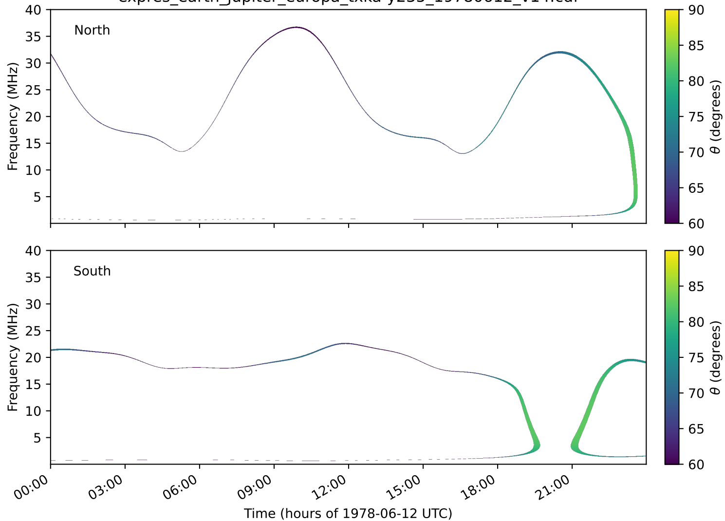
expres_earth_jupiter_europa_txka-y235_19780612_v14.cdf
