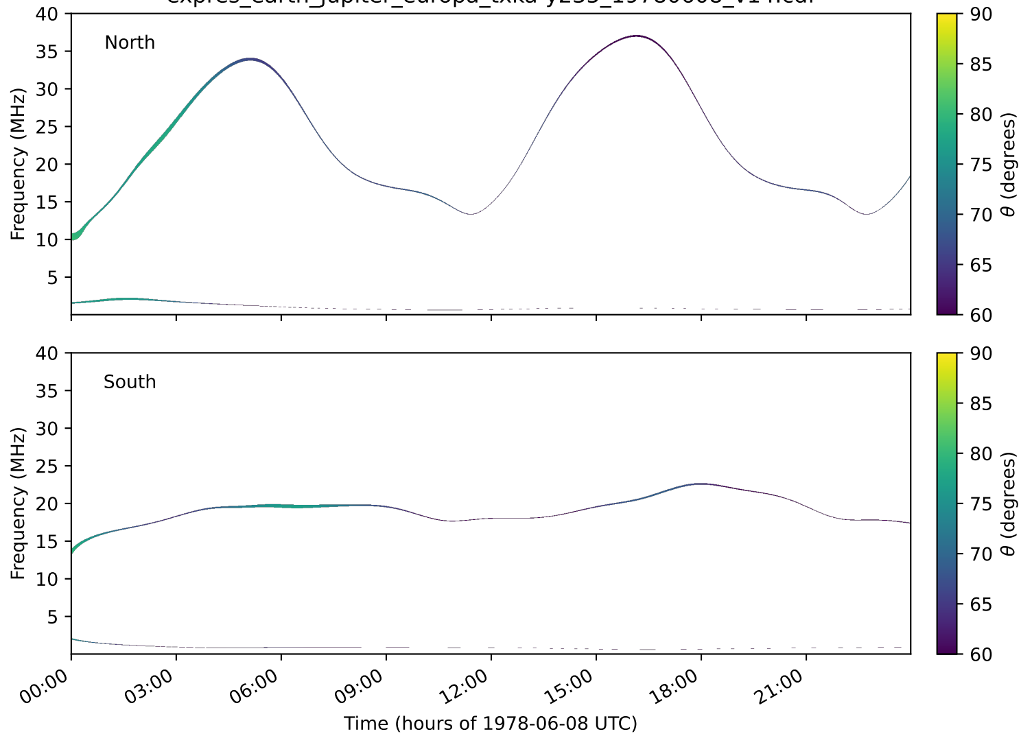
expres_earth_jupiter_europa_txka-y235_19780608_v14.cdf
