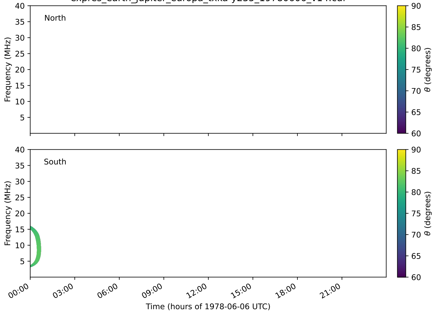
expres_earth_jupiter_europa_txka-y235_19780606_v14.cdf
