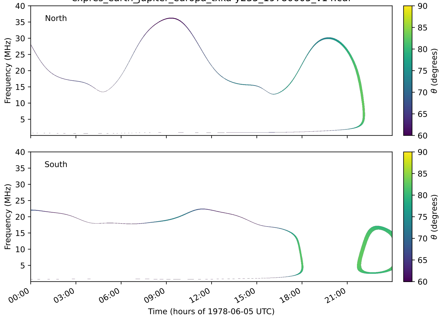
expres_earth_jupiter_europa_txka-y235_19780605_v14.cdf
