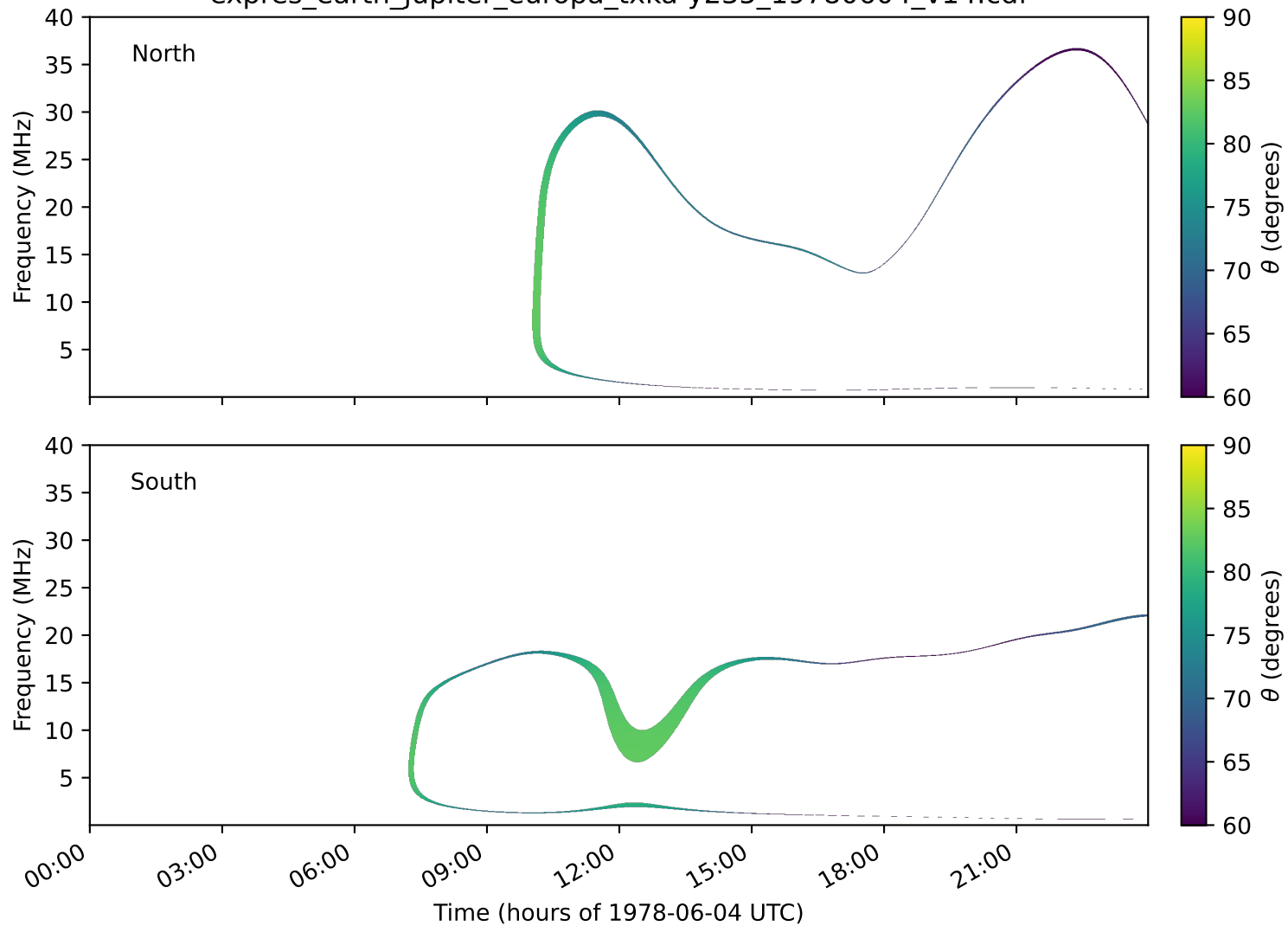
expres_earth_jupiter_europa_txka-y235_19780604_v14.cdf
