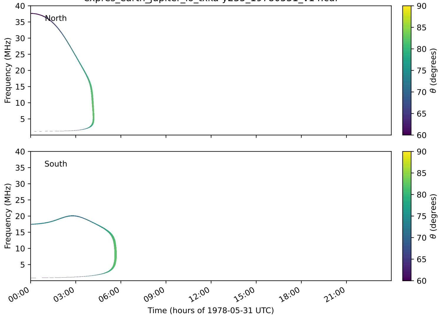
expres_earth_jupiter_io_txka-y235_19780531_v14.cdf
