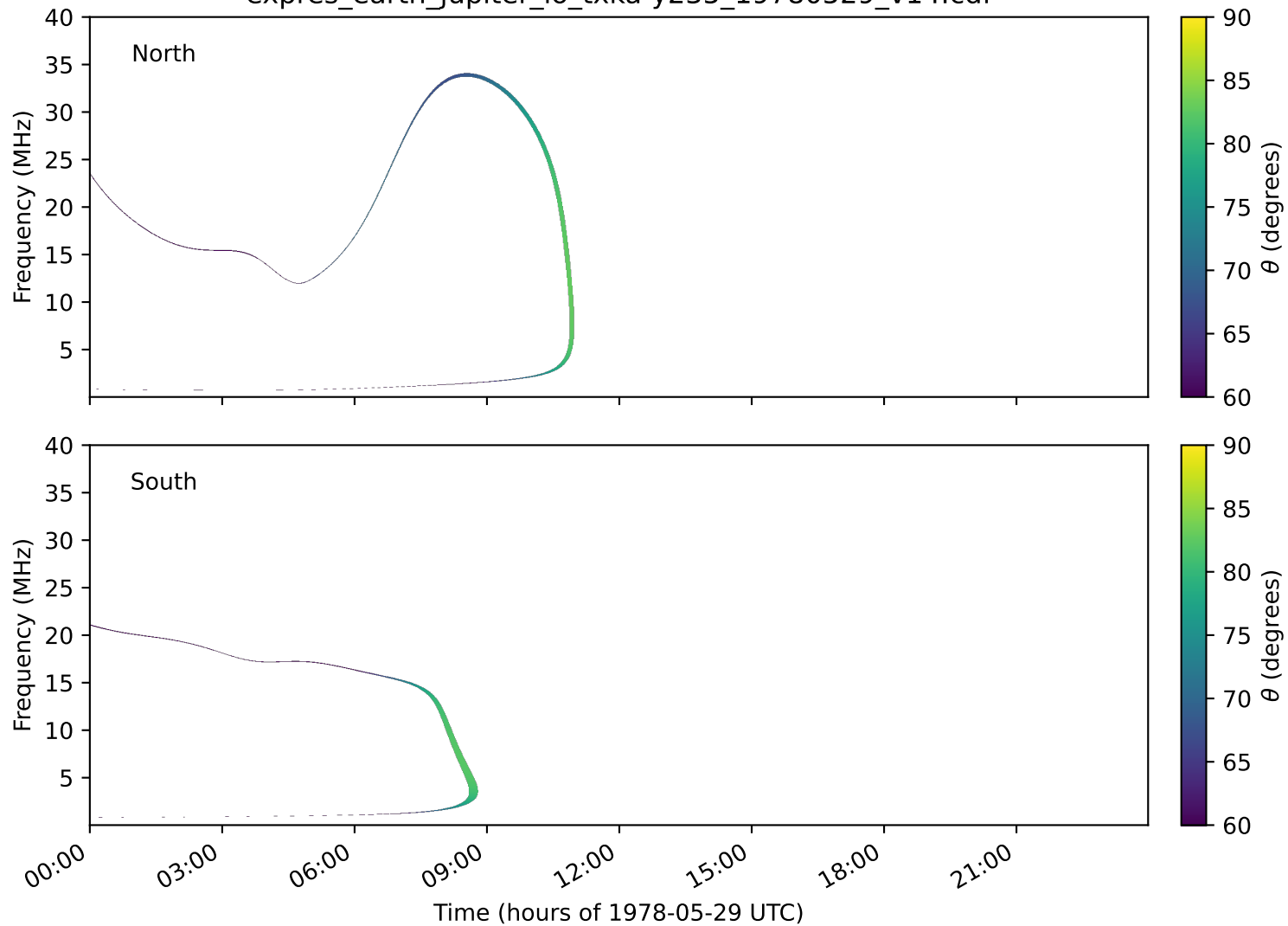
expres_earth_jupiter_io_txka-y235_19780529_v14.cdf
