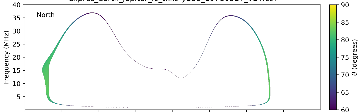
expres_earth_jupiter_io_txka-y235_19780527_v14.cdf
