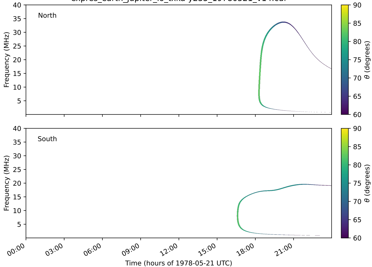
expres_earth_jupiter_io_txka-y235_19780521_v14.cdf
