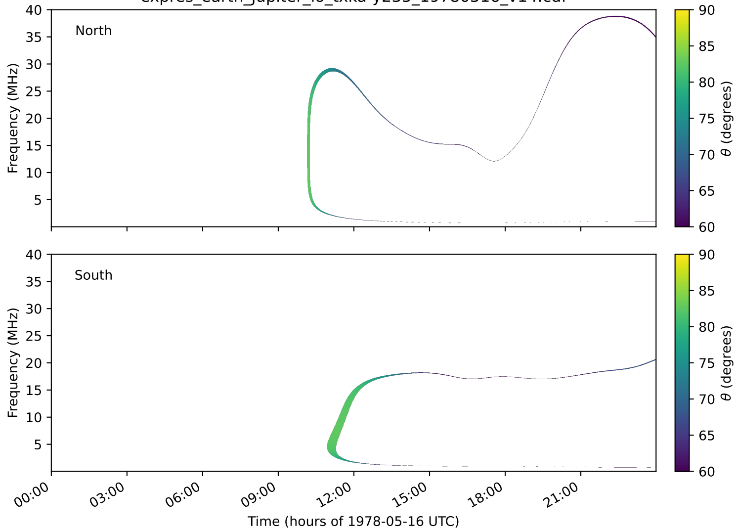
expres_earth_jupiter_io_txka-y235_19780516_v14.cdf
