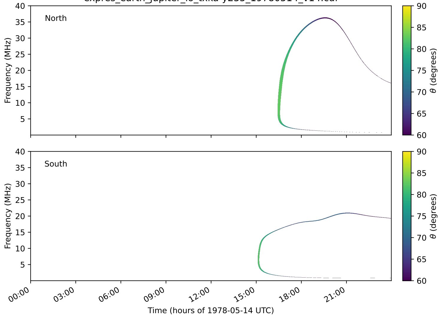
expres_earth_jupiter_io_txka-y235_19780514_v14.cdf
