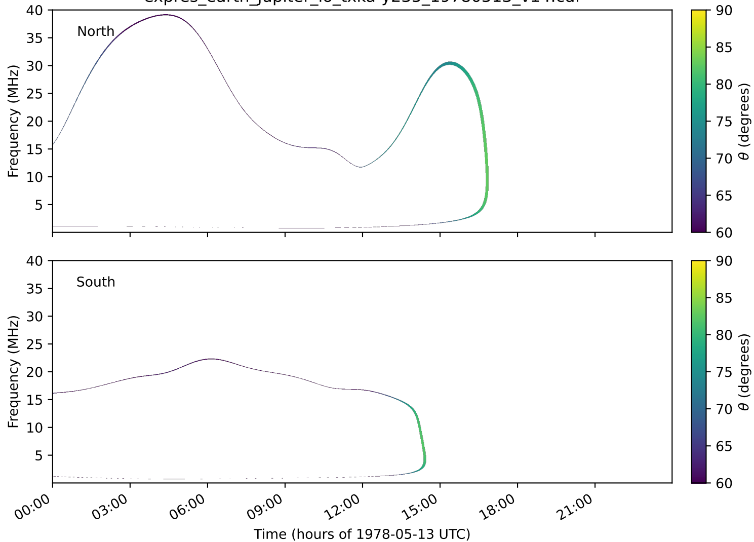
expres_earth_jupiter_io_txka-y235_19780513_v14.cdf
