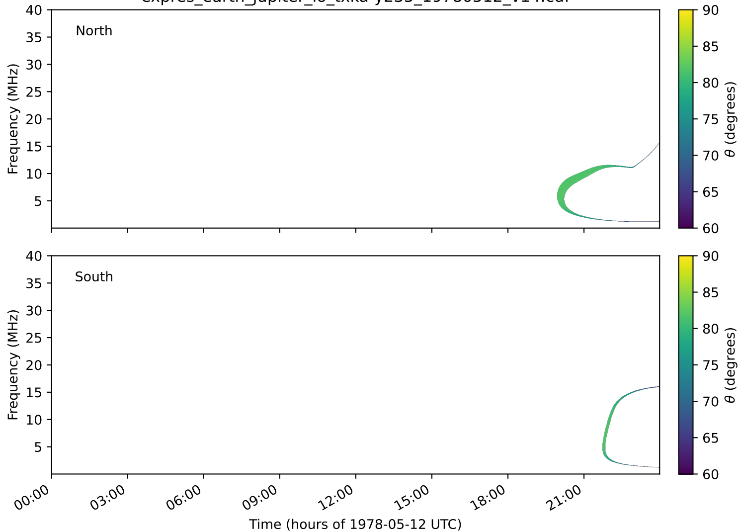
expres_earth_jupiter_io_txka-y235_19780512_v14.cdf
