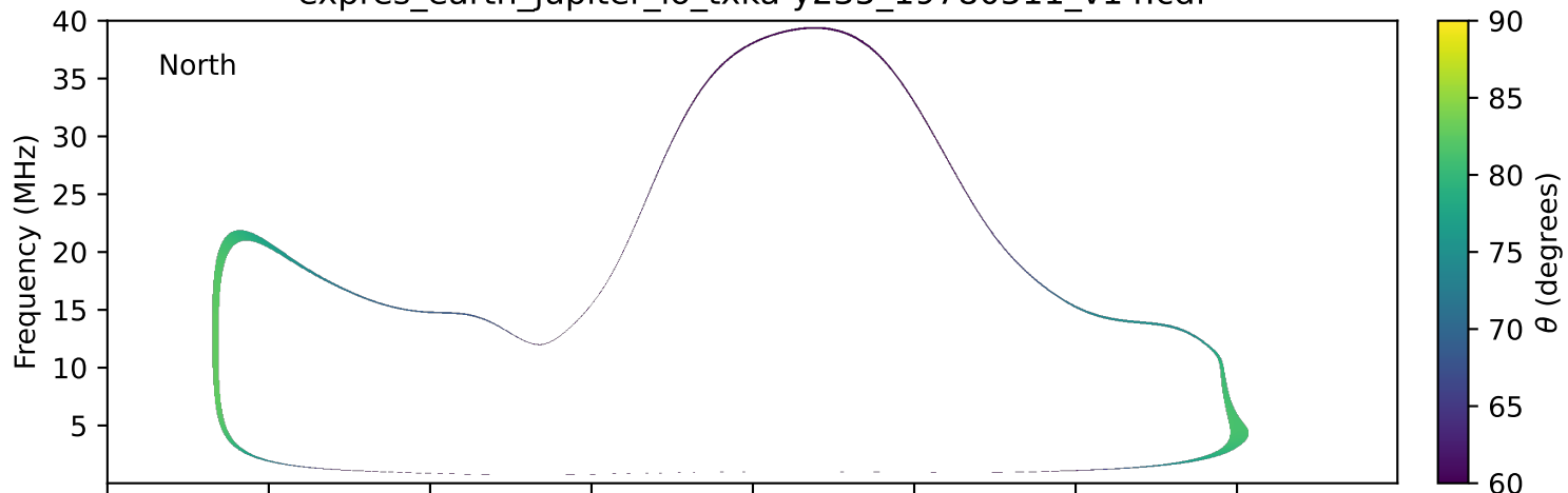
expres_earth_jupiter_io_txka-y235_19780511_v14.cdf
