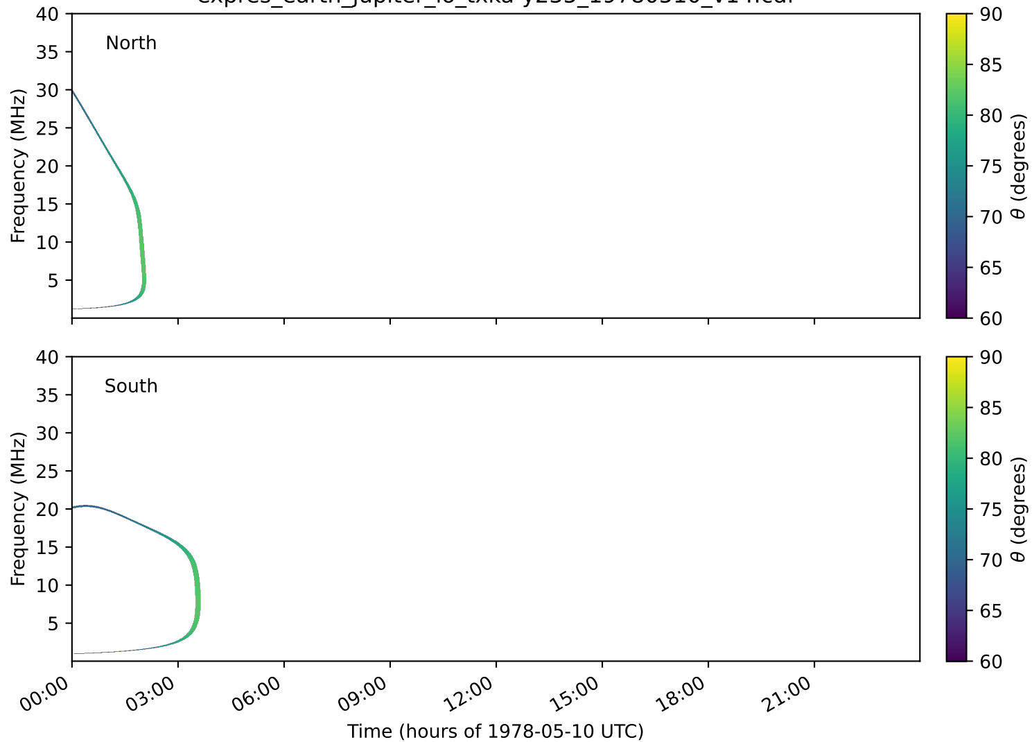
expres_earth_jupiter_io_txka-y235_19780510_v14.cdf
