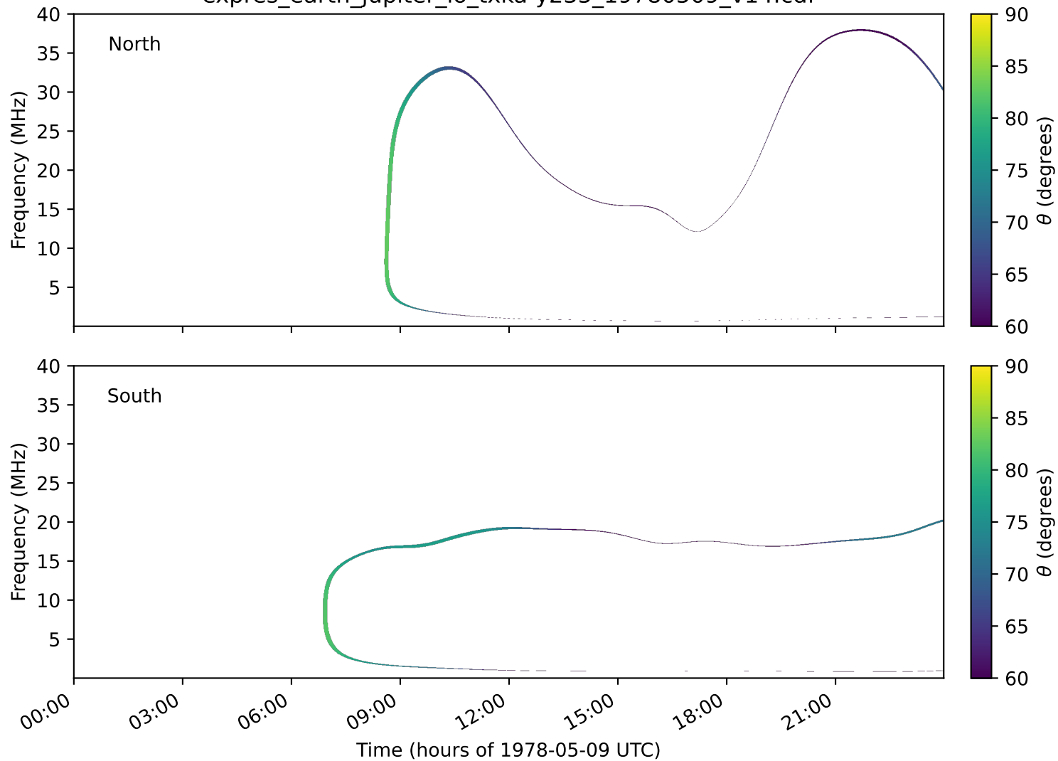
expres_earth_jupiter_io_txka-y235_19780509_v14.cdf
