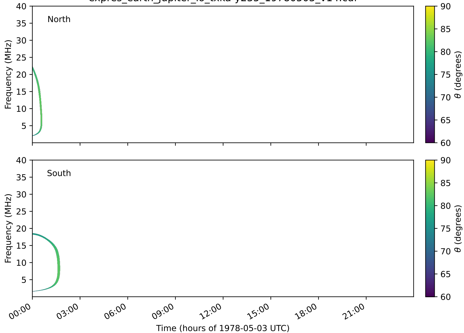
expres_earth_jupiter_io_txka-y235_19780503_v14.cdf
