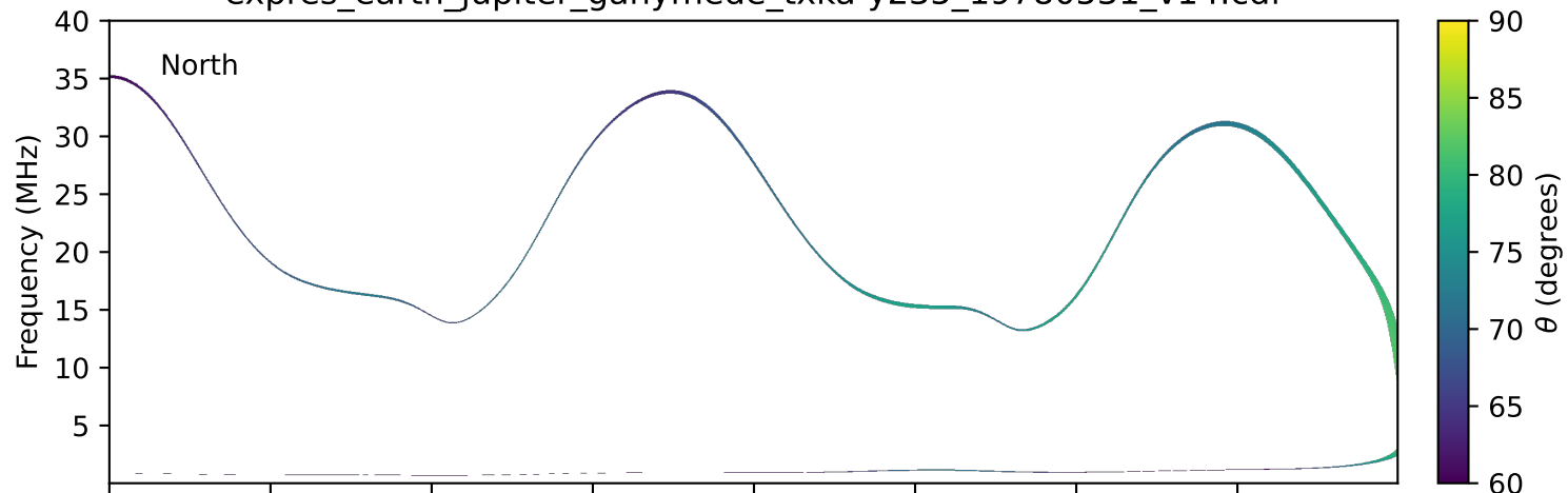
expres_earth_jupiter_ganymede_txka-y235_19780531_v14.cdf
