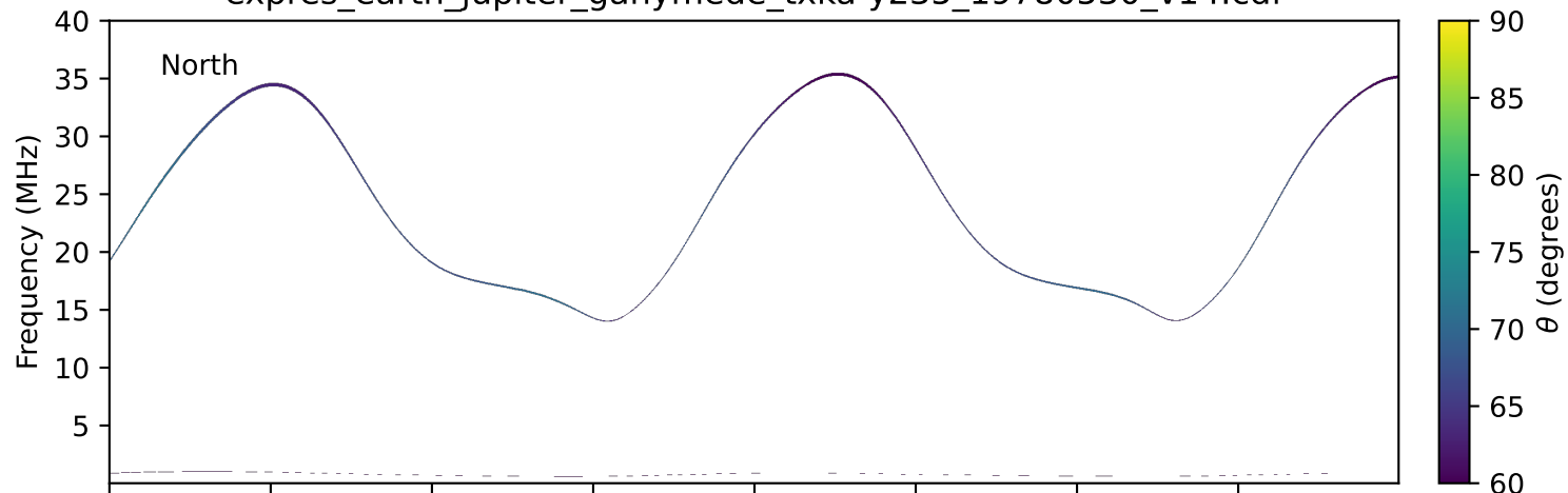
expres_earth_jupiter_ganymede_txka-y235_19780530_v14.cdf
