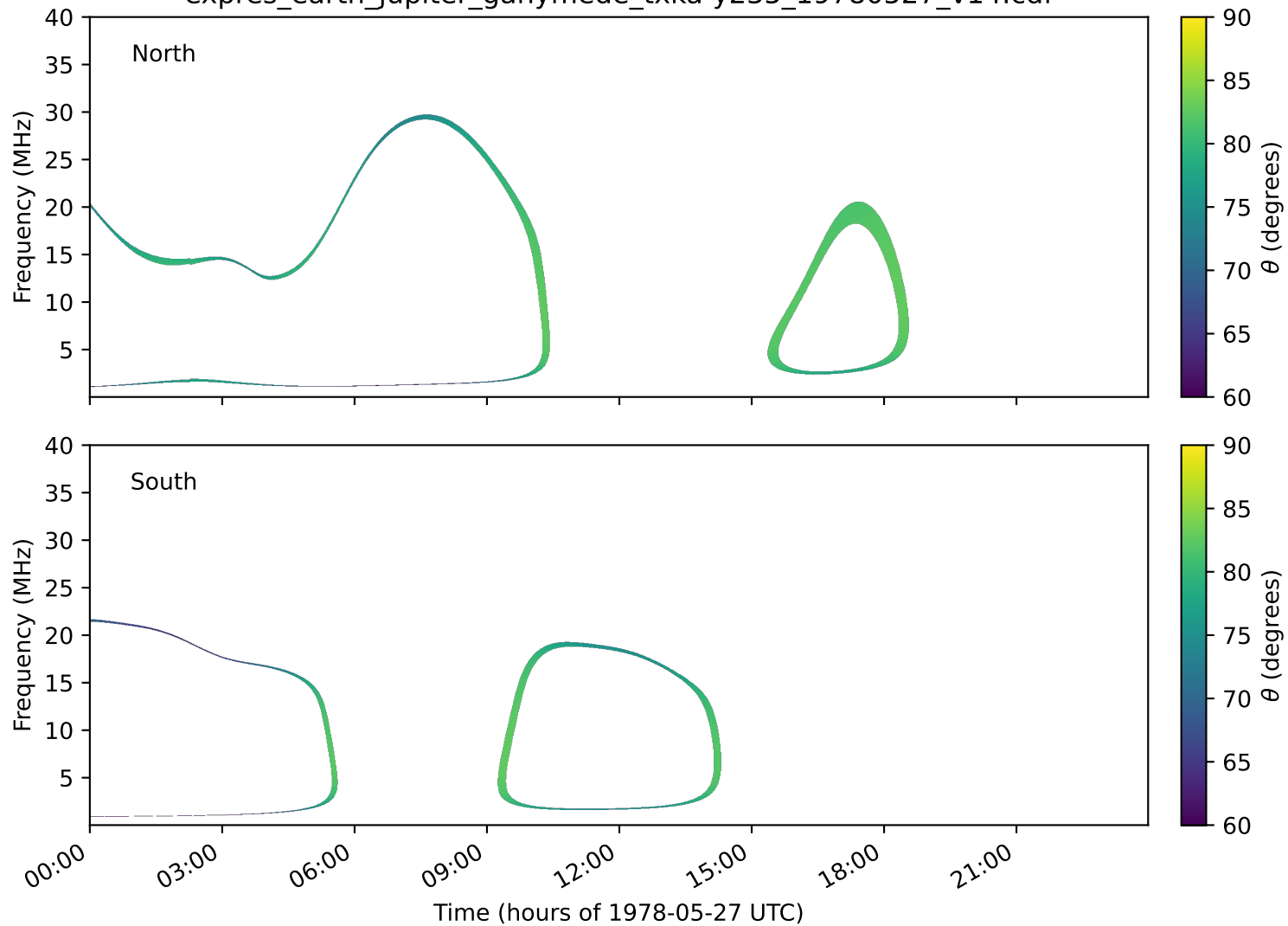
expres_earth_jupiter_ganymede_txka-y235_19780527_v14.cdf
