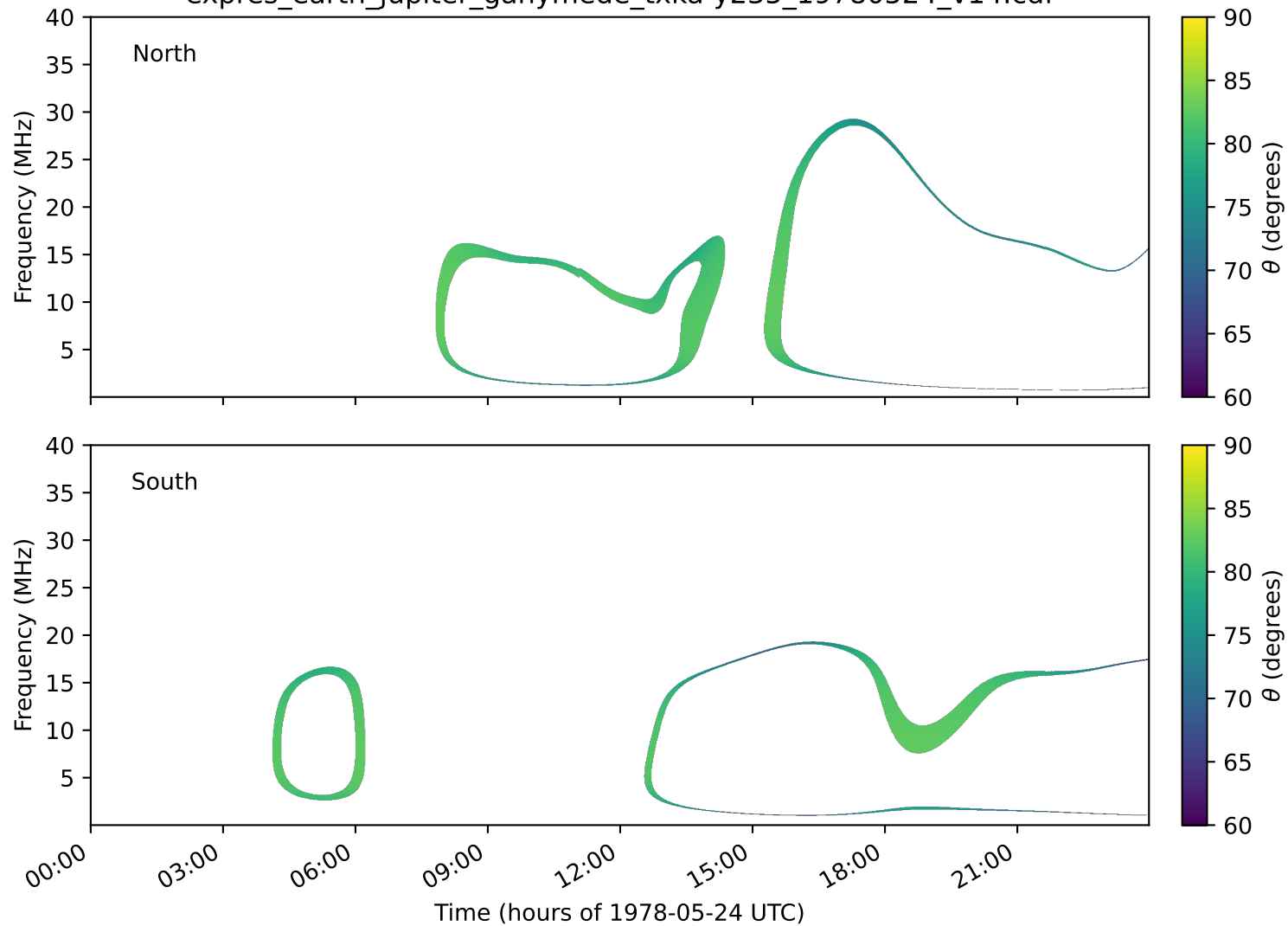
expres_earth_jupiter_ganymede_txka-y235_19780524_v14.cdf
