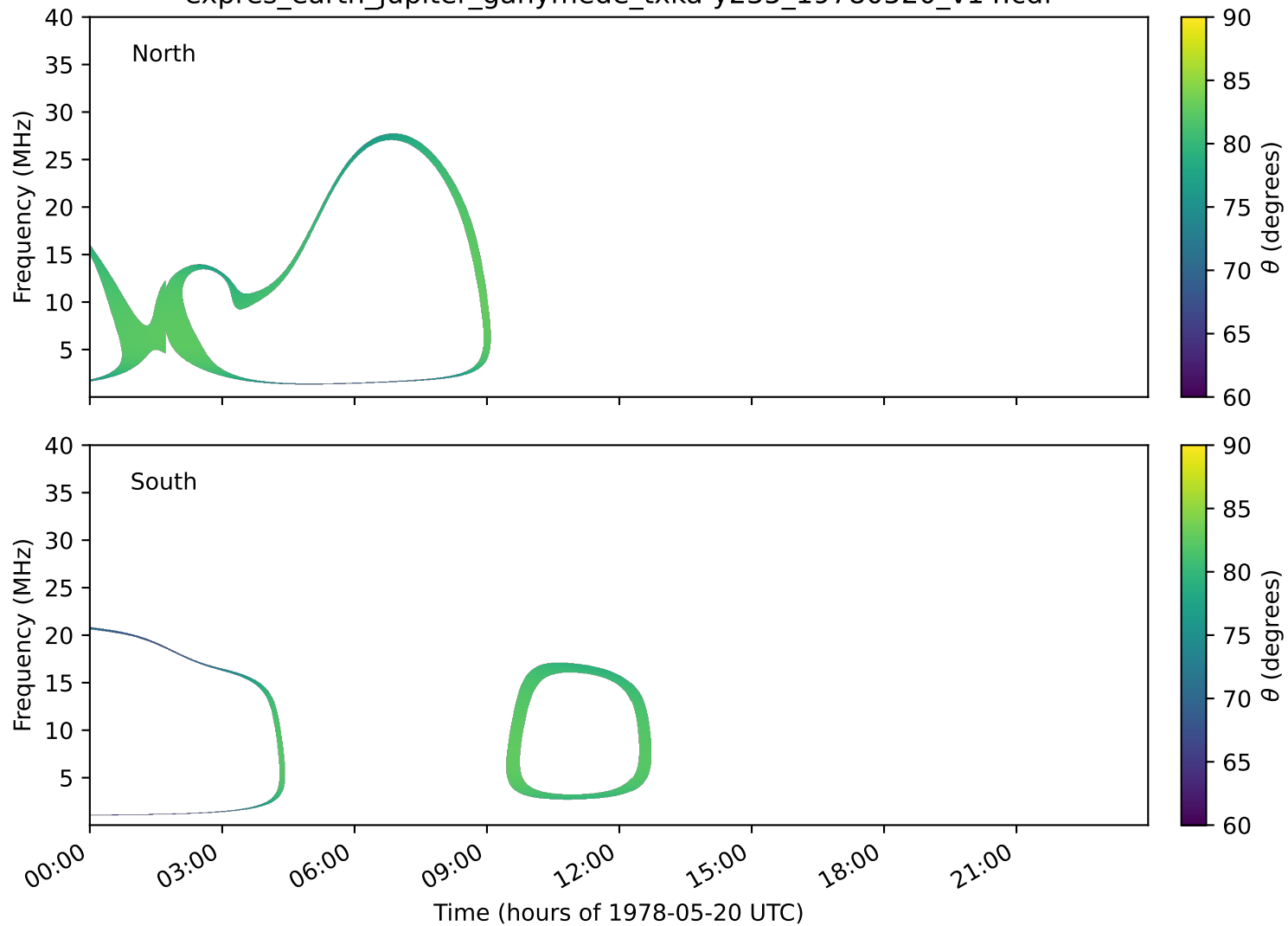
expres_earth_jupiter_ganymede_txka-y235_19780520_v14.cdf
