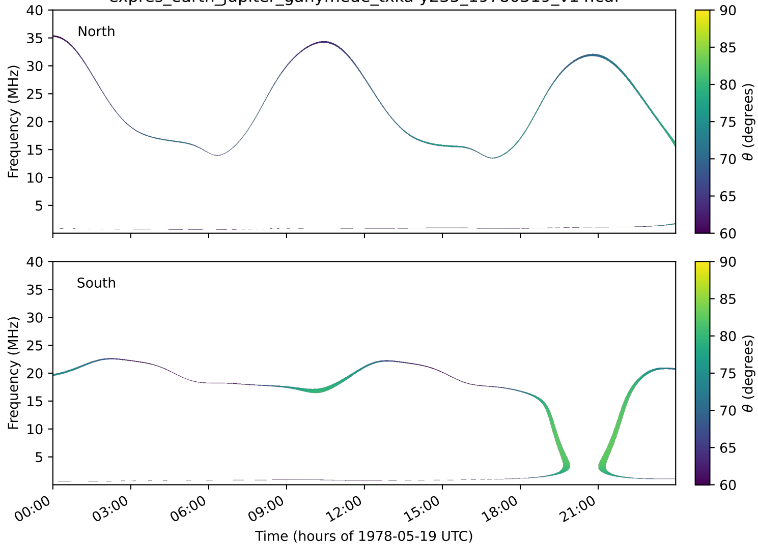
expres_earth_jupiter_ganymede_txka-y235_19780519_v14.cdf
