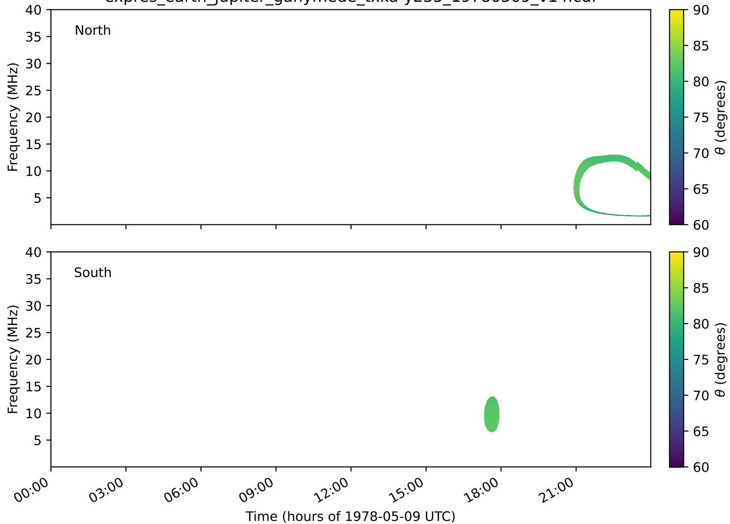
expres_earth_jupiter_ganymede_txka-y235_19780509_v14.cdf
