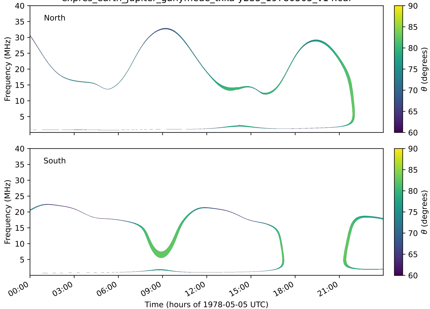
expres_earth_jupiter_ganymede_txka-y235_19780505_v14.cdf
