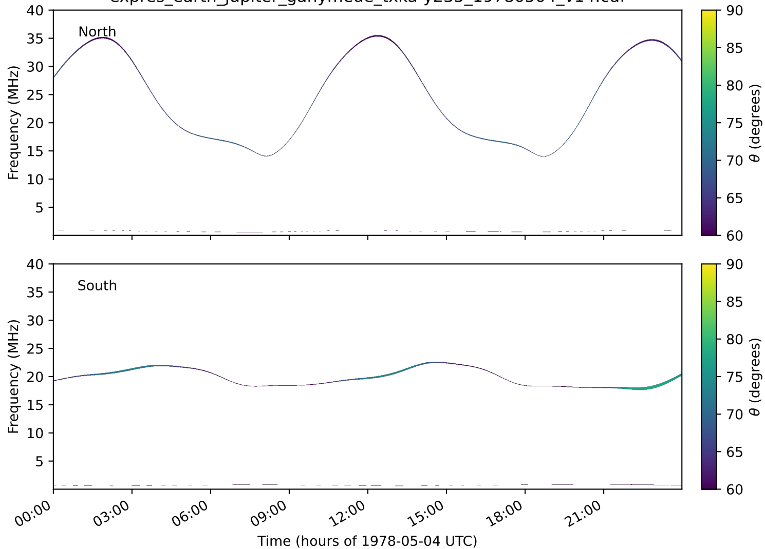
expres_earth_jupiter_ganymede_txka-y235_19780504_v14.cdf
