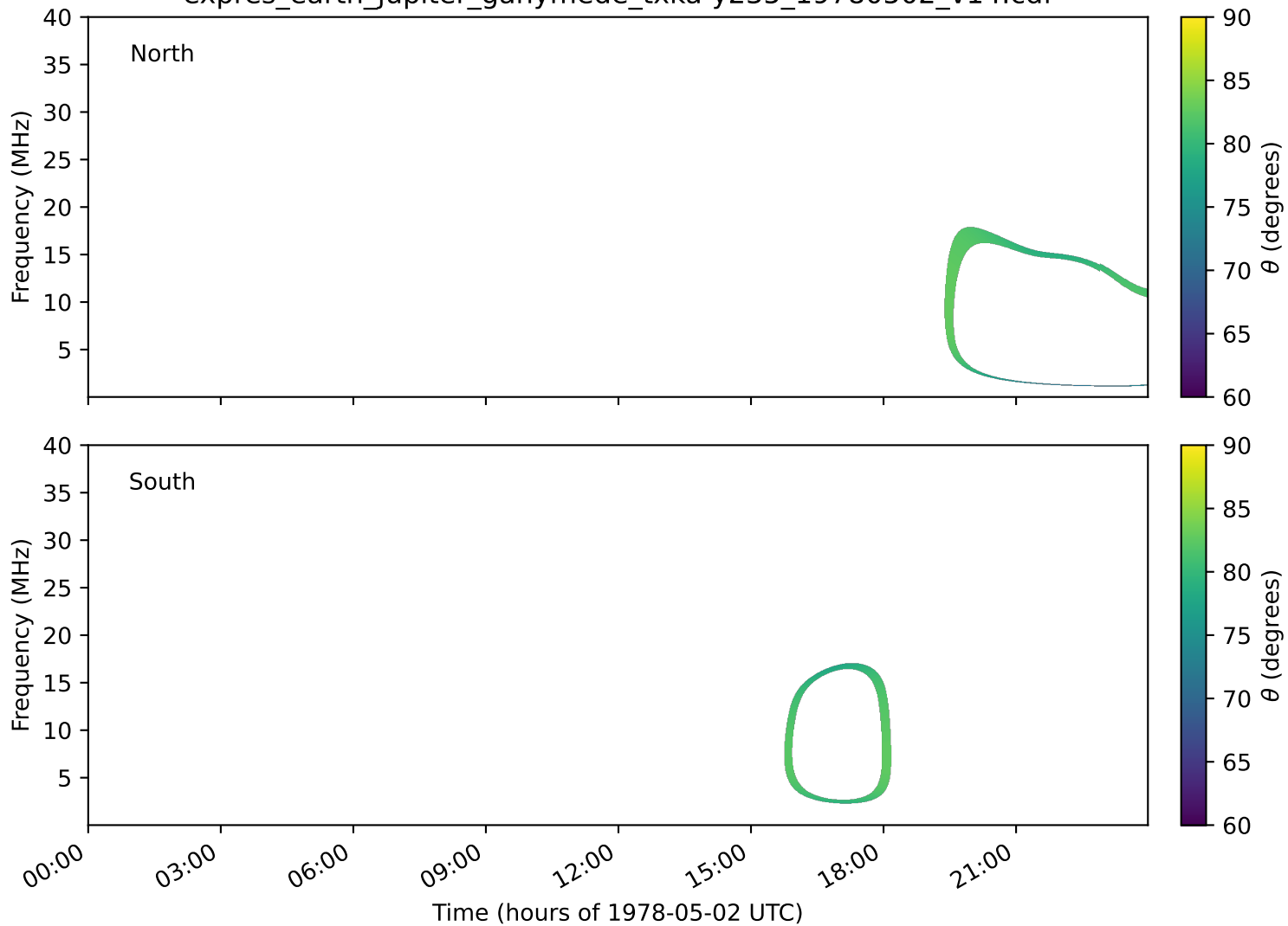
expres_earth_jupiter_ganymede_txka-y235_19780502_v14.cdf
