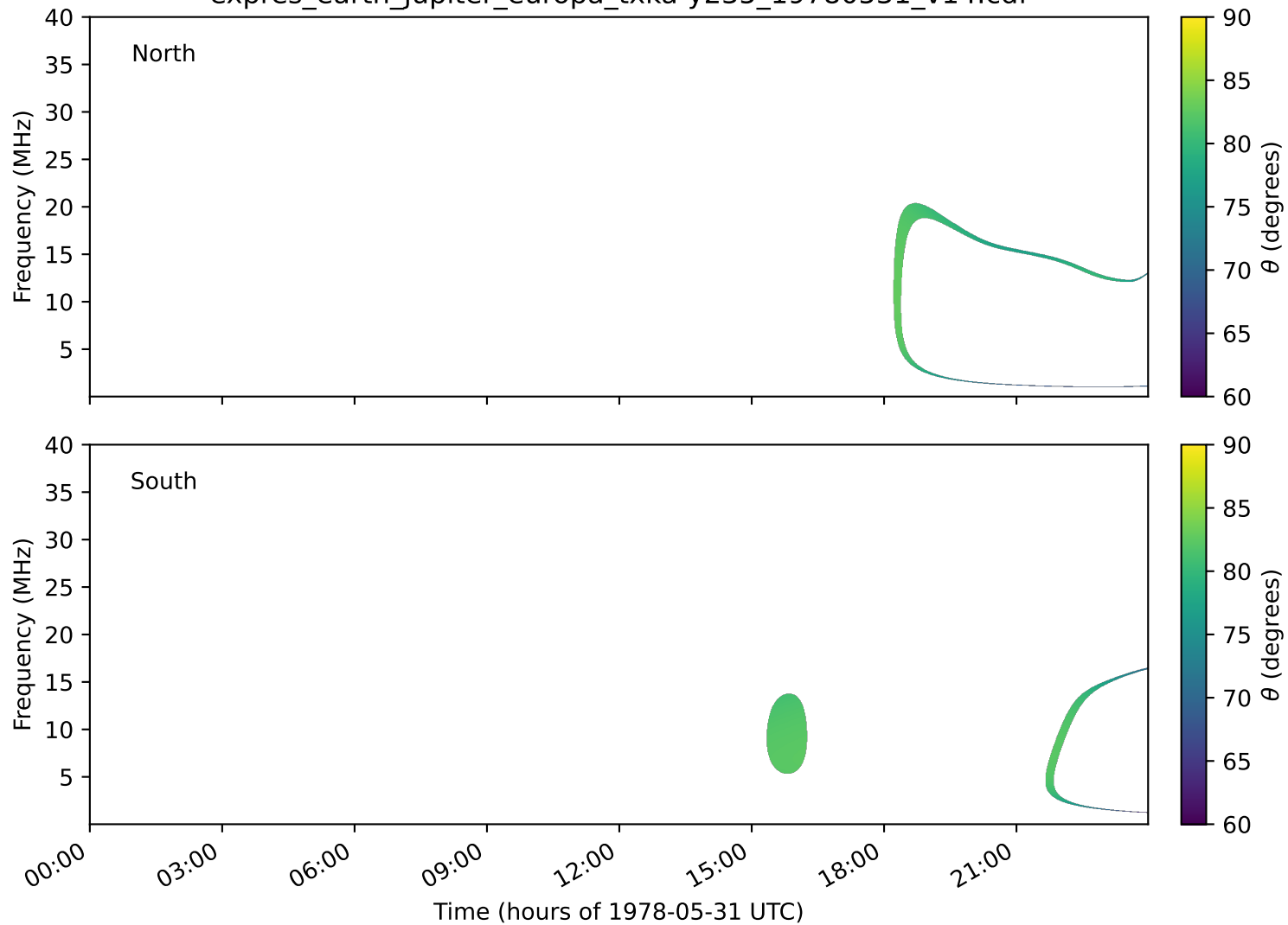
expres_earth_jupiter_europa_txka-y235_19780531_v14.cdf
