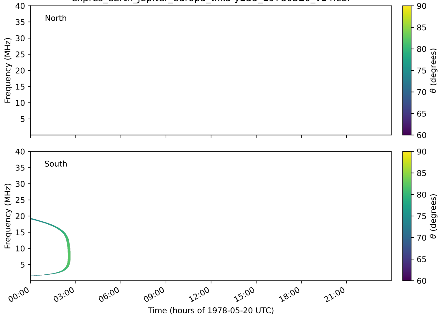
expres_earth_jupiter_europa_txka-y235_19780520_v14.cdf
