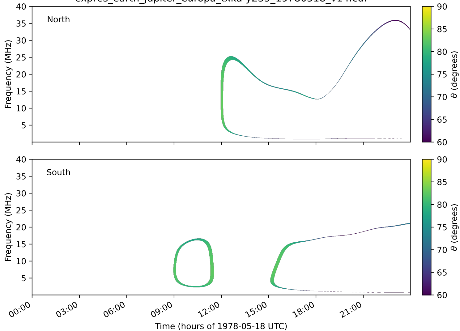
expres_earth_jupiter_europa_txka-y235_19780518_v14.cdf
