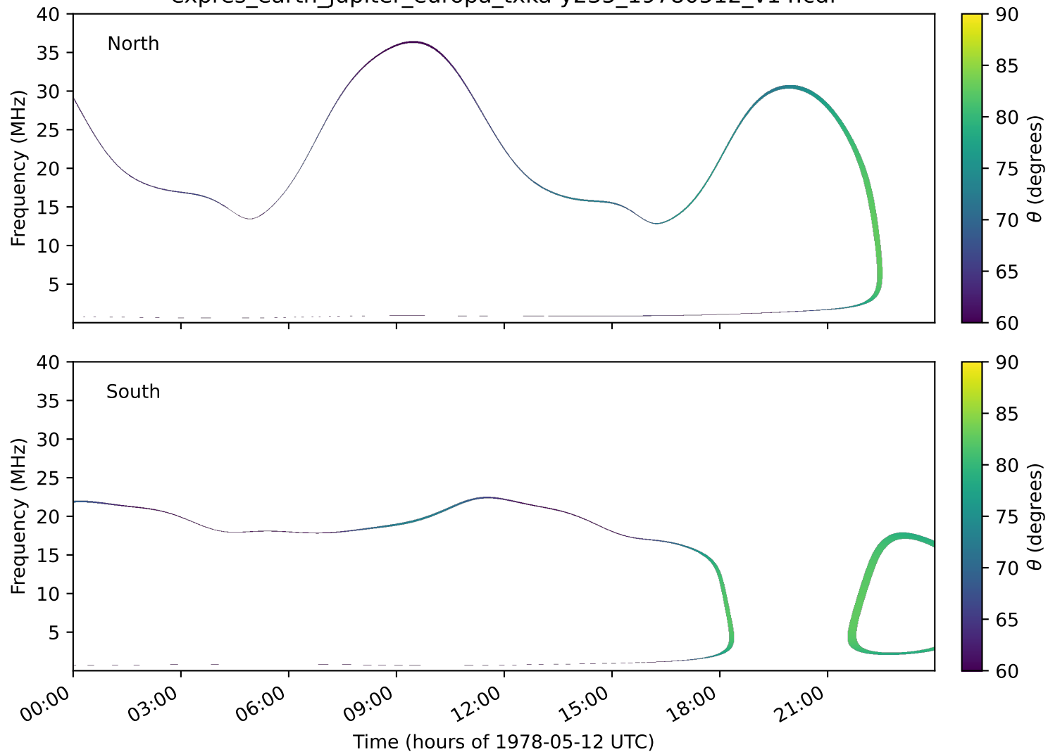
expres_earth_jupiter_europa_txka-y235_19780512_v14.cdf
