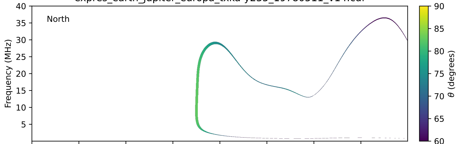
expres_earth_jupiter_europa_txka-y235_19780511_v14.cdf
