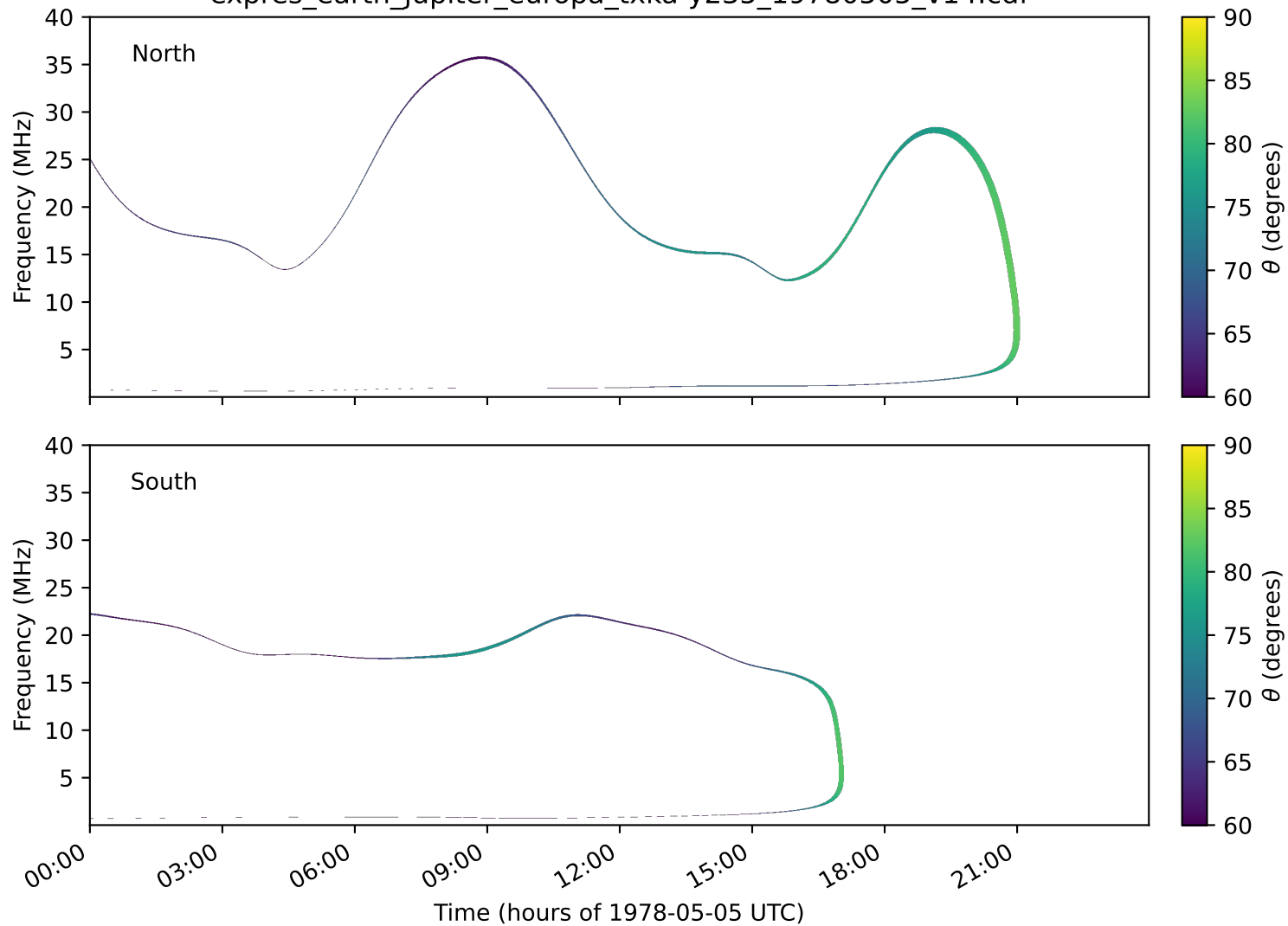
expres_earth_jupiter_europa_txka-y235_19780505_v14.cdf
