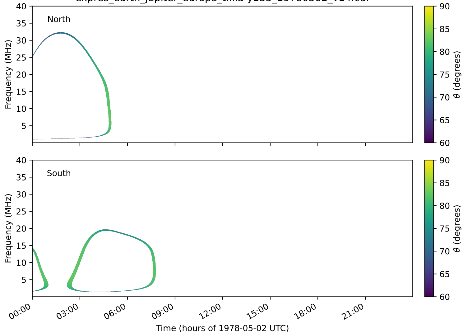
expres_earth_jupiter_europa_txka-y235_19780502_v14.cdf
