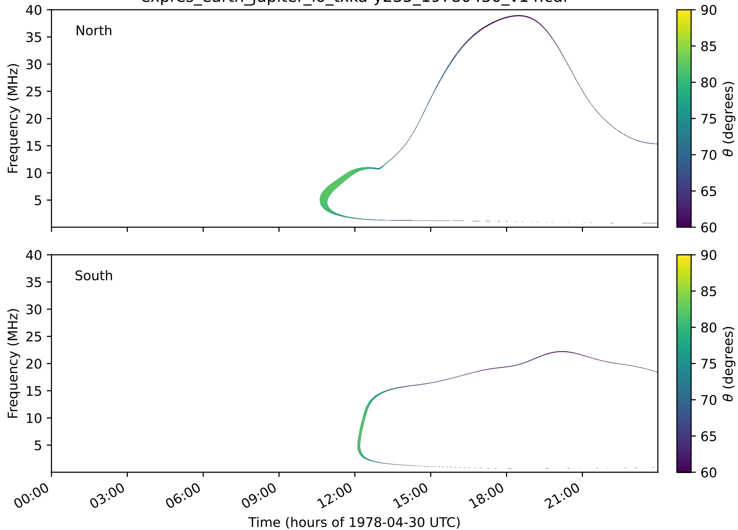
expres_earth_jupiter_io_txka-y235_19780430_v14.cdf
