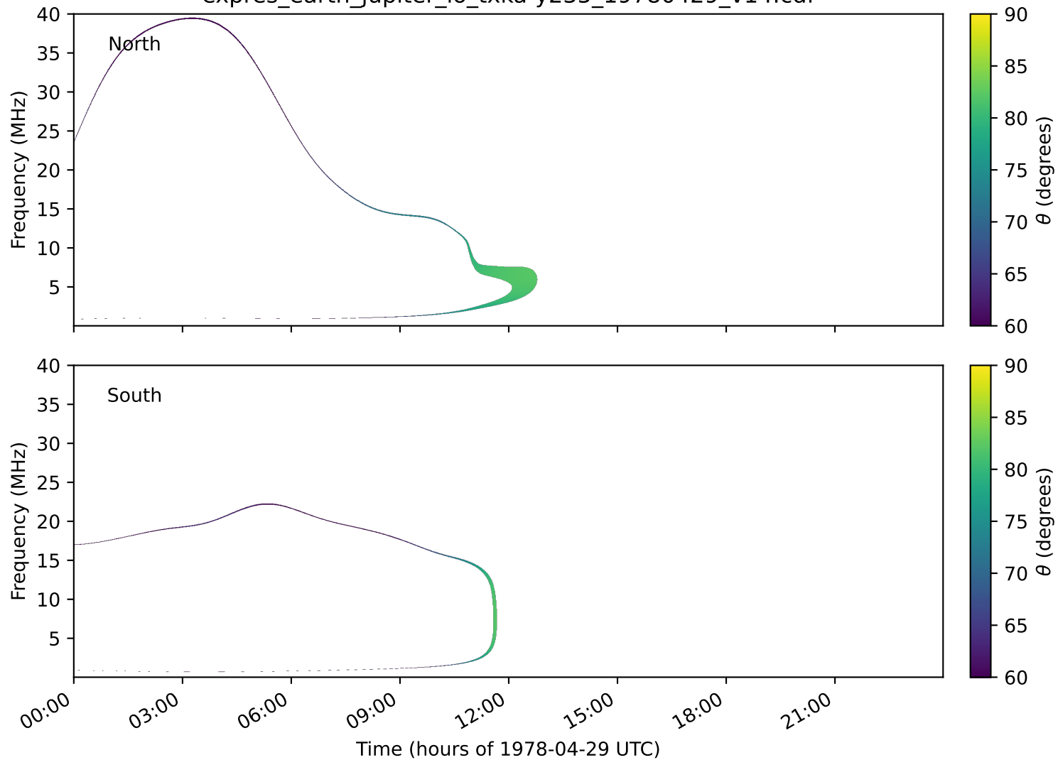
expres_earth_jupiter_io_txka-y235_19780429_v14.cdf
