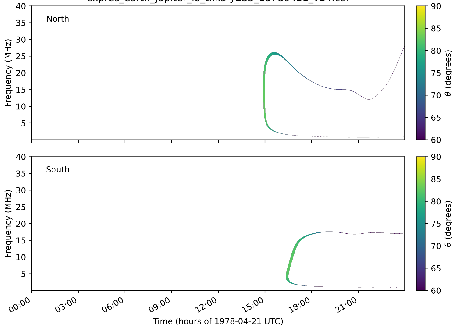
expres_earth_jupiter_io_txka-y235_19780421_v14.cdf
