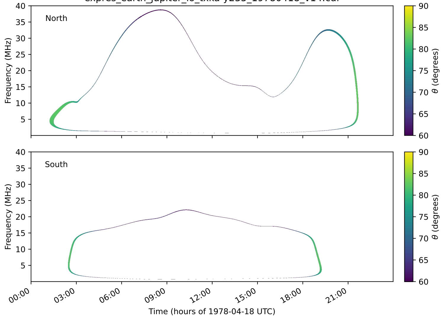
expres_earth_jupiter_io_txka-y235_19780418_v14.cdf
