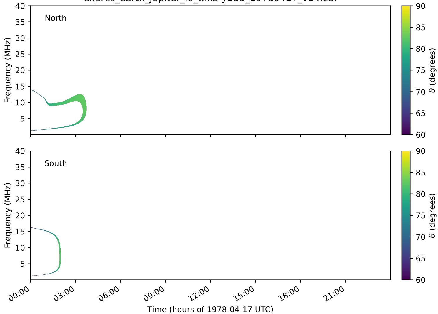
expres_earth_jupiter_io_txka-y235_19780417_v14.cdf
