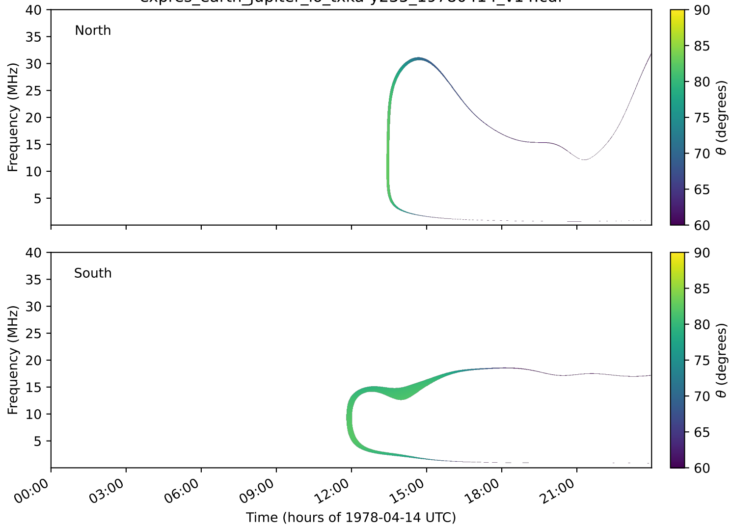
expres_earth_jupiter_io_txka-y235_19780414_v14.cdf
